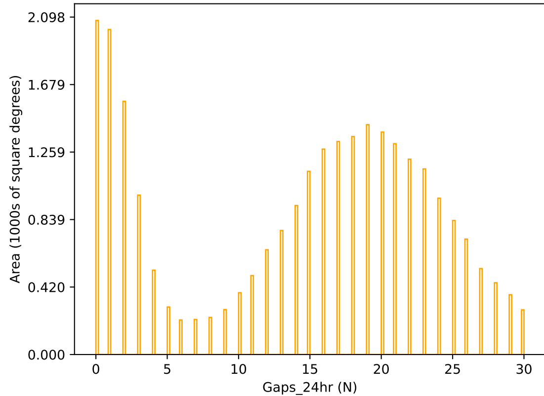
baseline_v3.3_10yrs r band: Gaps_24hr
