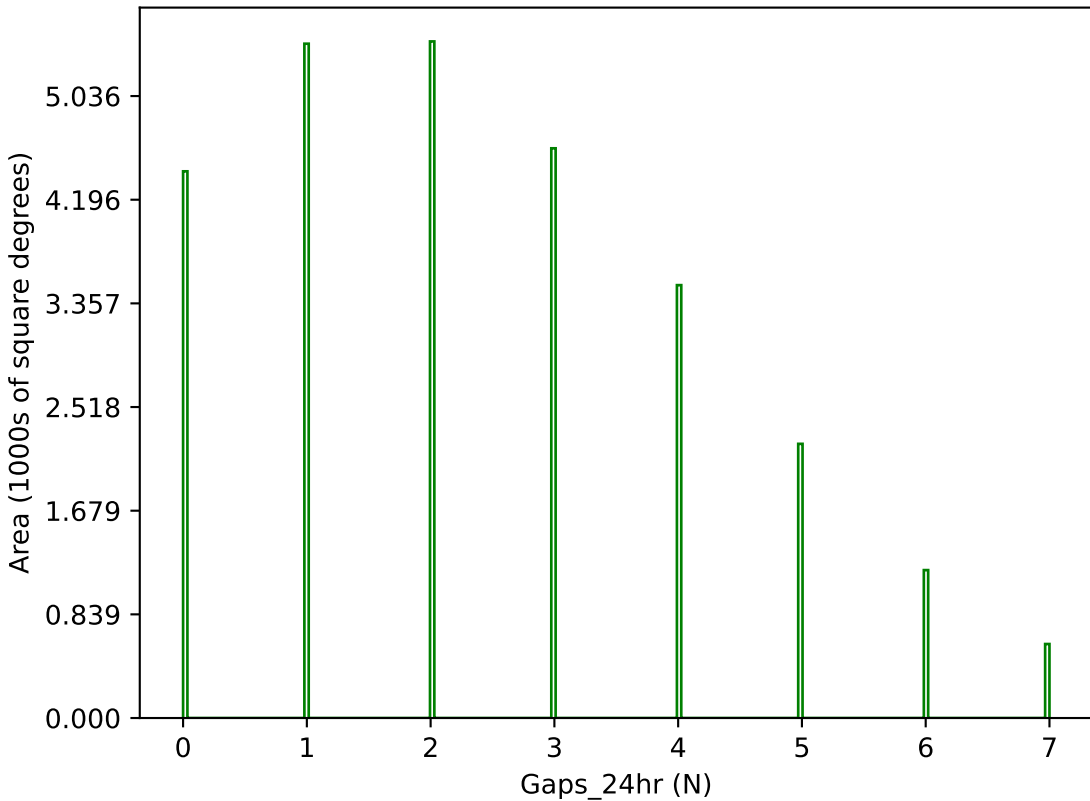
baseline_v3.3_10yrs g band: Gaps_24hr
