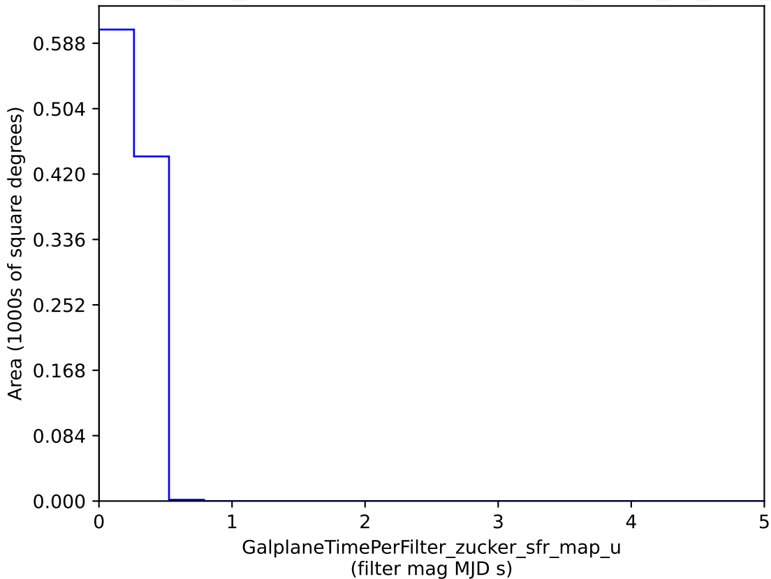
baseline_v3.3_10yrs : GalplaneTimePerFilter_zucker_sfr_map_u
