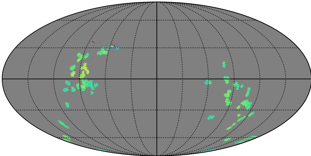
baseline_v3.3_10yrs : GalplaneTimePerFilter_zucker_sfr_map_r
