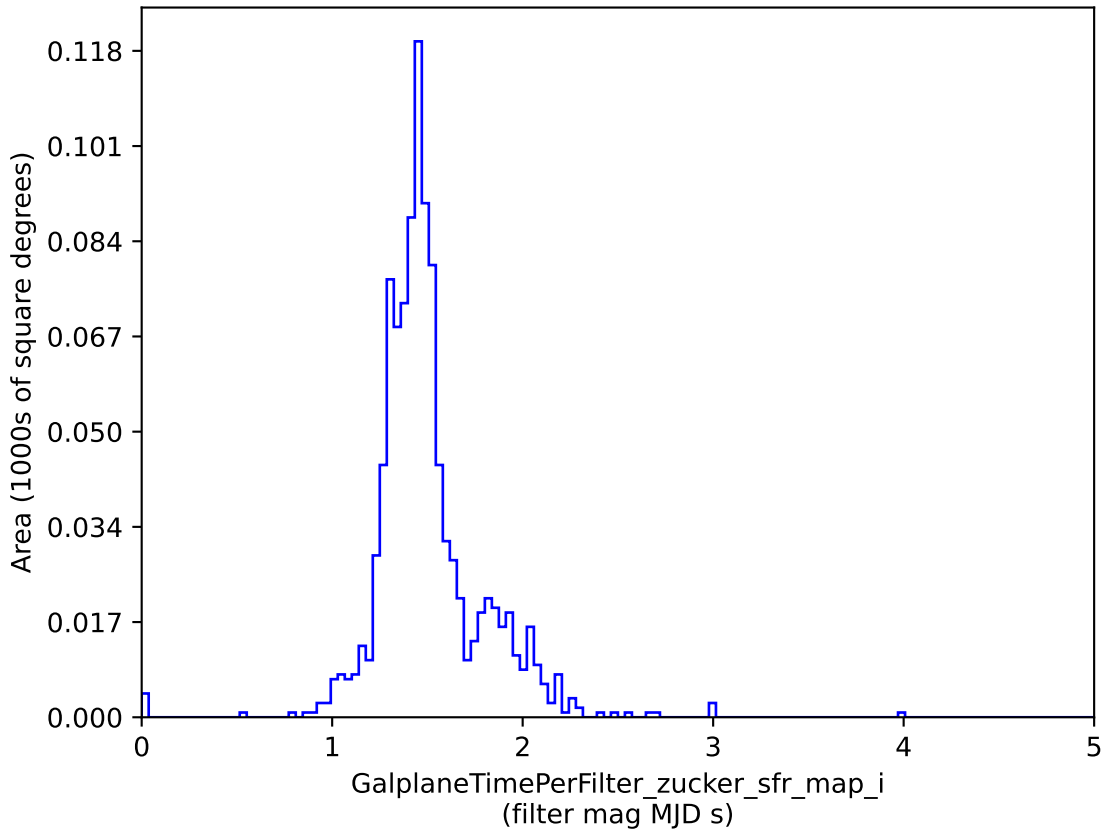
baseline_v3.3_10yrs : GalplaneTimePerFilter_zucker_sfr_map_i
