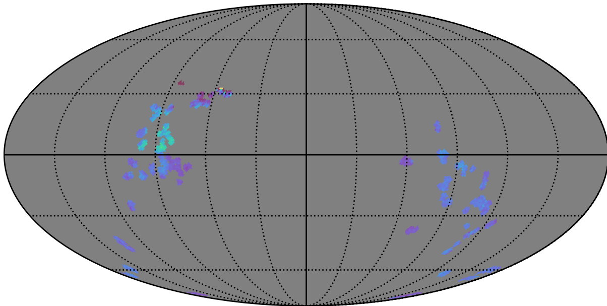
baseline_v3.3_10yrs : GalplaneTimePerFilter_zucker_sfr_map_g
