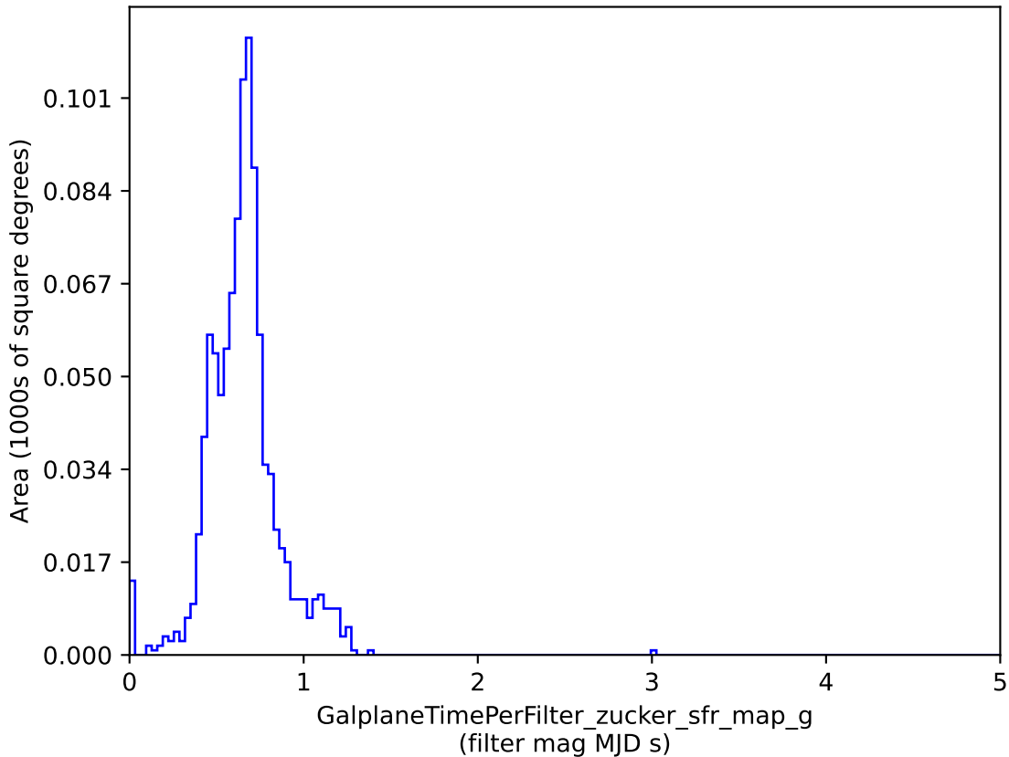
baseline_v3.3_10yrs : GalplaneTimePerFilter_zucker_sfr_map_g
