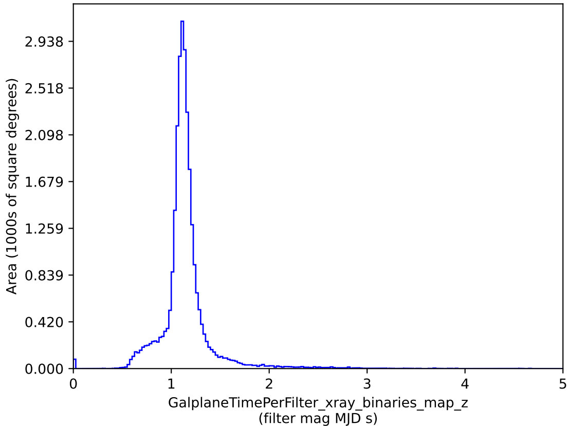
baseline_v3.3_10yrs : GalplaneTimePerFilter_xray_binaries_map_z
