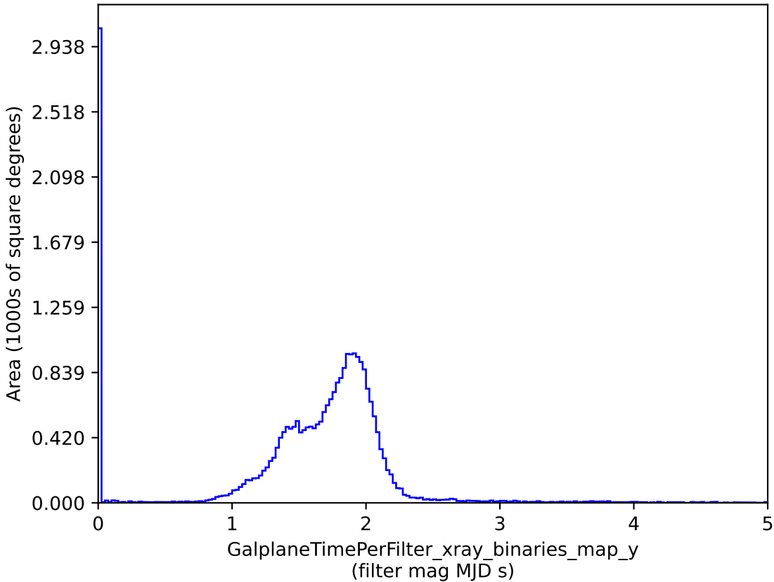
baseline_v3.3_10yrs : GalplaneTimePerFilter_xray_binaries_map_y
