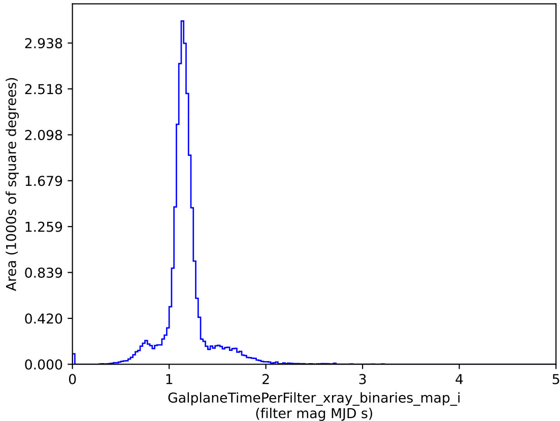
baseline_v3.3_10yrs : GalplaneTimePerFilter_xray_binaries_map_i
