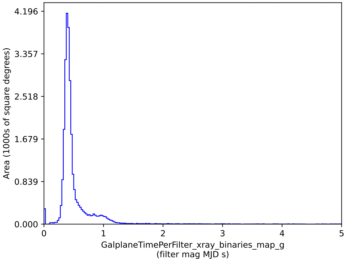
baseline_v3.3_10yrs : GalplaneTimePerFilter_xray_binaries_map_g
