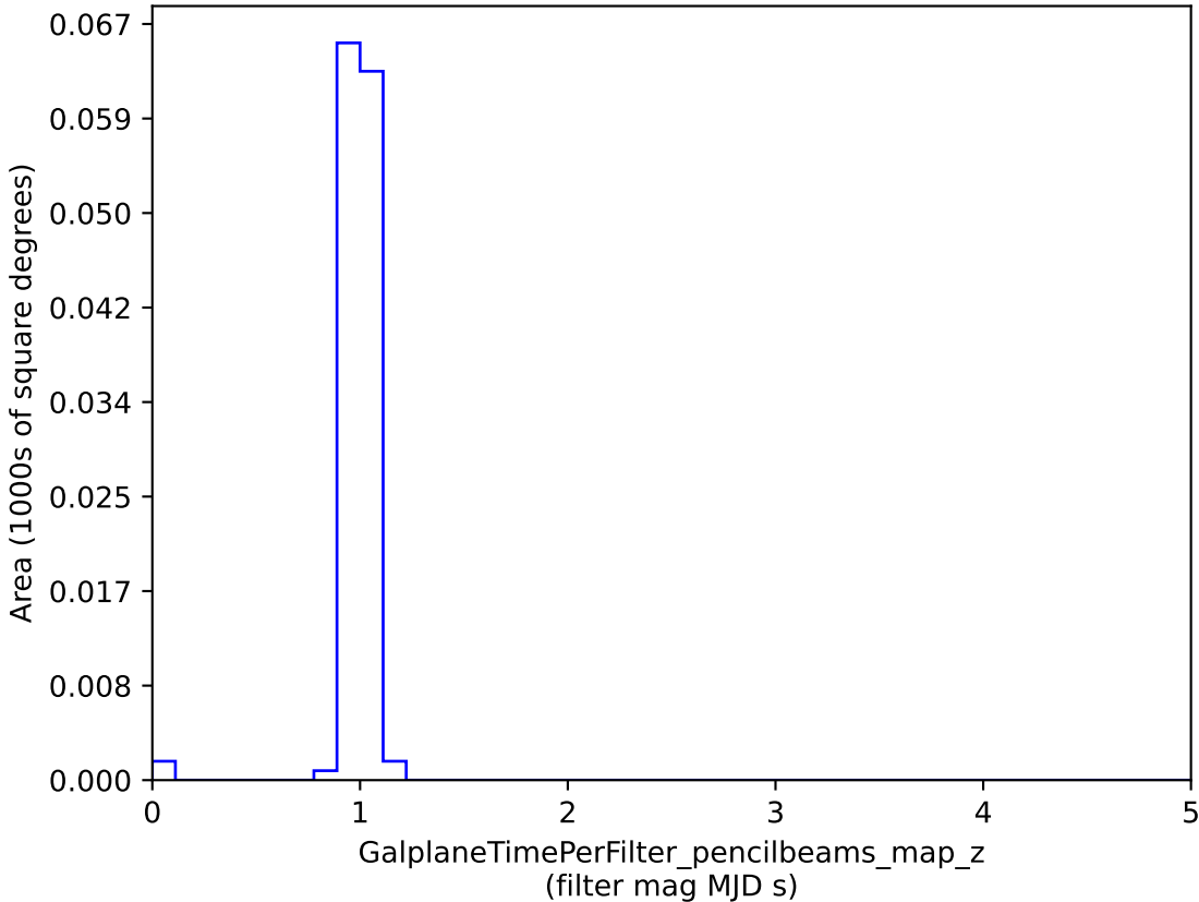
baseline_v3.3_10yrs : GalplaneTimePerFilter_pencilbeams_map_z
