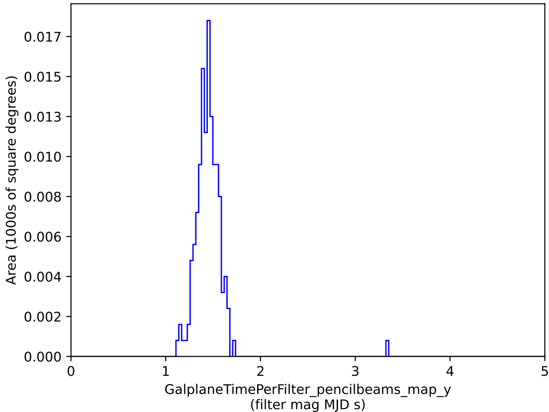
baseline_v3.3_10yrs : GalplaneTimePerFilter_pencilbeams_map_y
