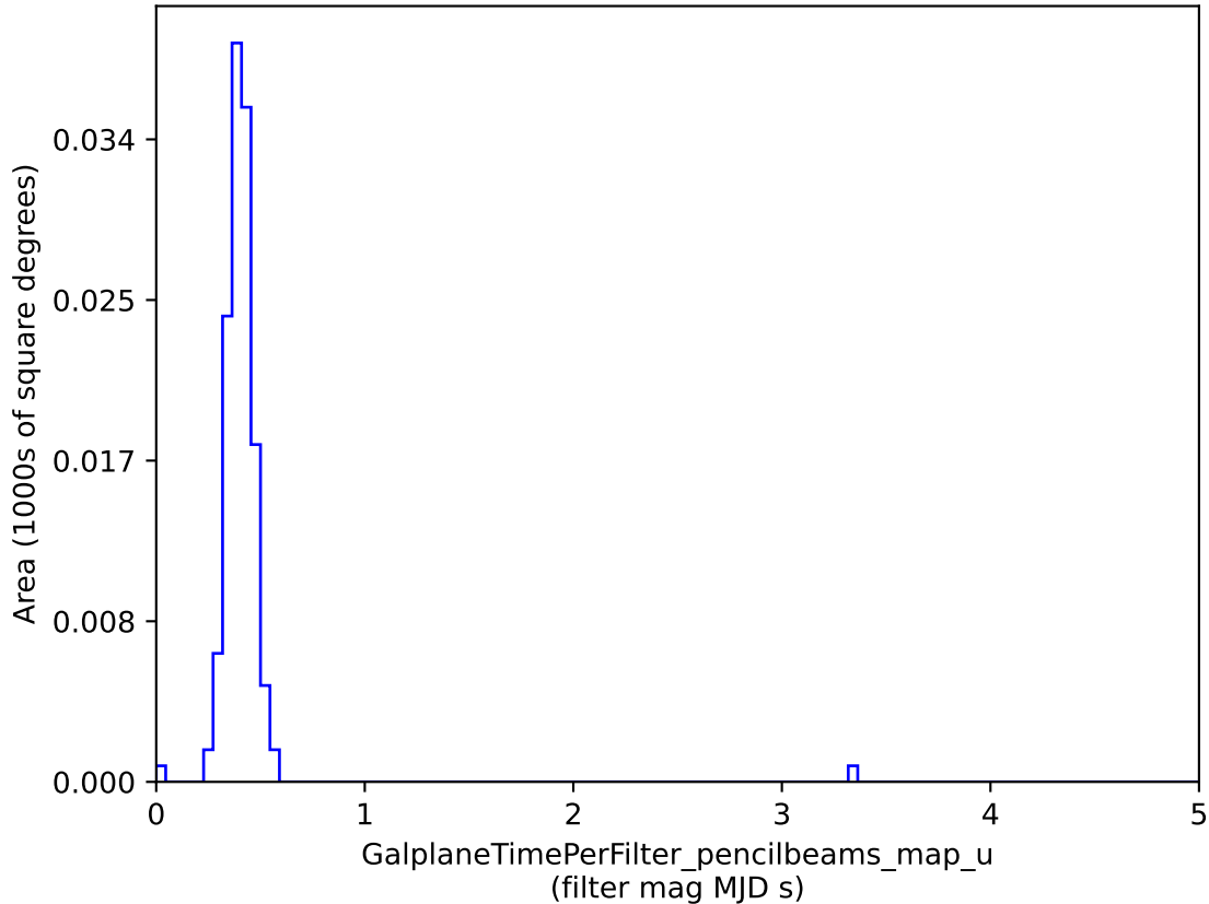
baseline_v3.3_10yrs : GalplaneTimePerFilter_pencilbeams_map_u
