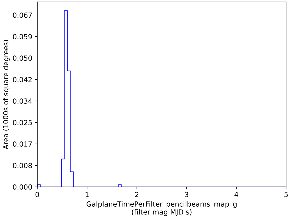
baseline_v3.3_10yrs : GalplaneTimePerFilter_pencilbeams_map_g
