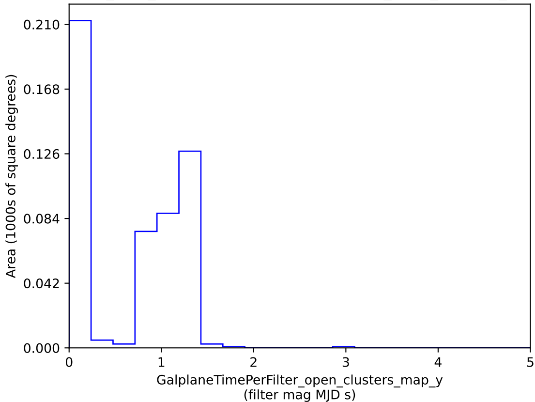
baseline_v3.3_10yrs : GalplaneTimePerFilter_open_clusters_map_y
