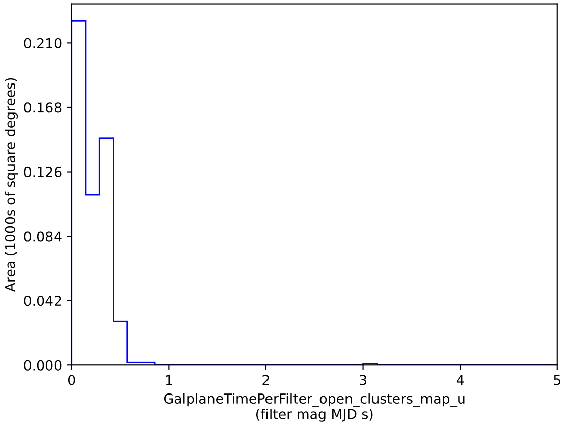
baseline_v3.3_10yrs : GalplaneTimePerFilter_open_clusters_map_u
