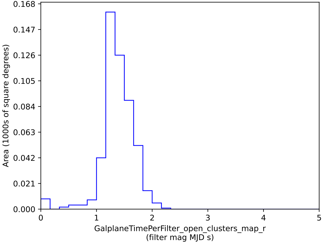
baseline_v3.3_10yrs : GalplaneTimePerFilter_open_clusters_map_r
