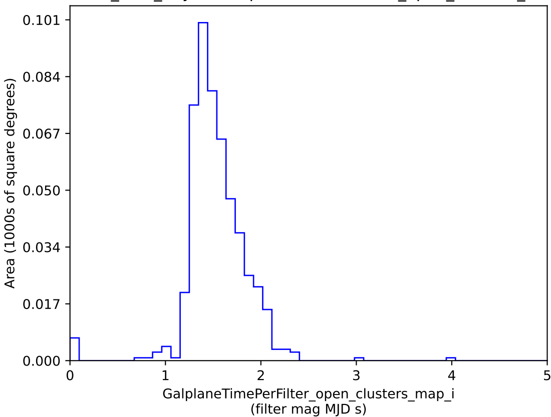
baseline_v3.3_10yrs : GalplaneTimePerFilter_open_clusters_map_i
