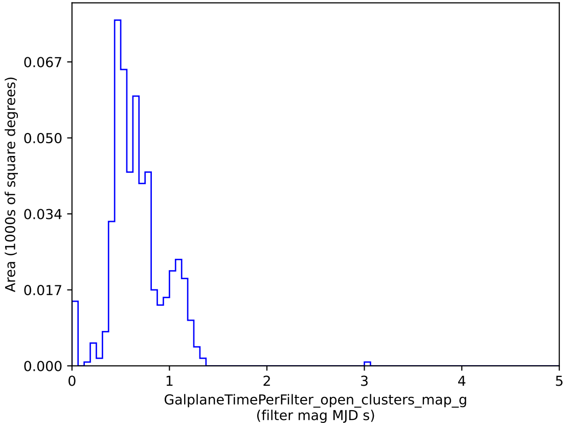
baseline_v3.3_10yrs : GalplaneTimePerFilter_open_clusters_map_g
