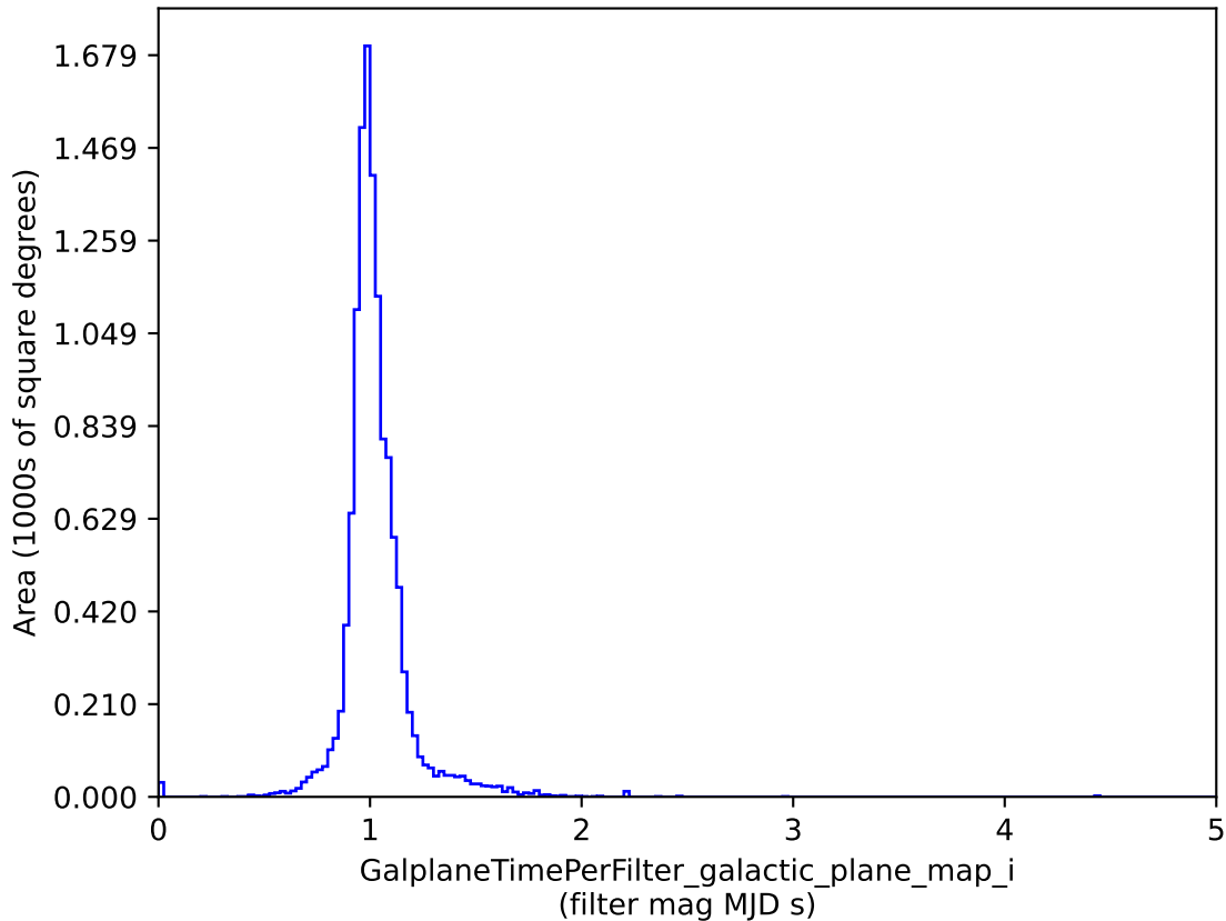
baseline_v3.3_10yrs : GalplaneTimePerFilter_galactic_plane_map_i
