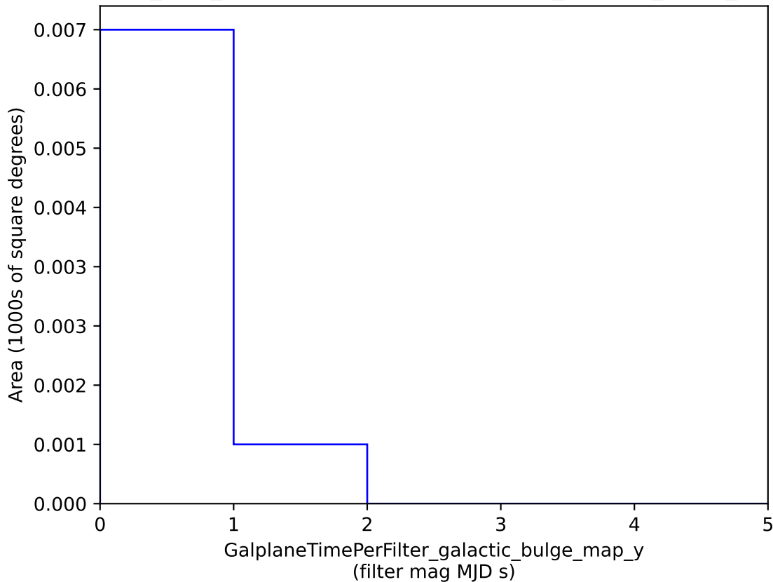
baseline_v3.3_10yrs : GalplaneTimePerFilter_galactic_bulge_map_y
