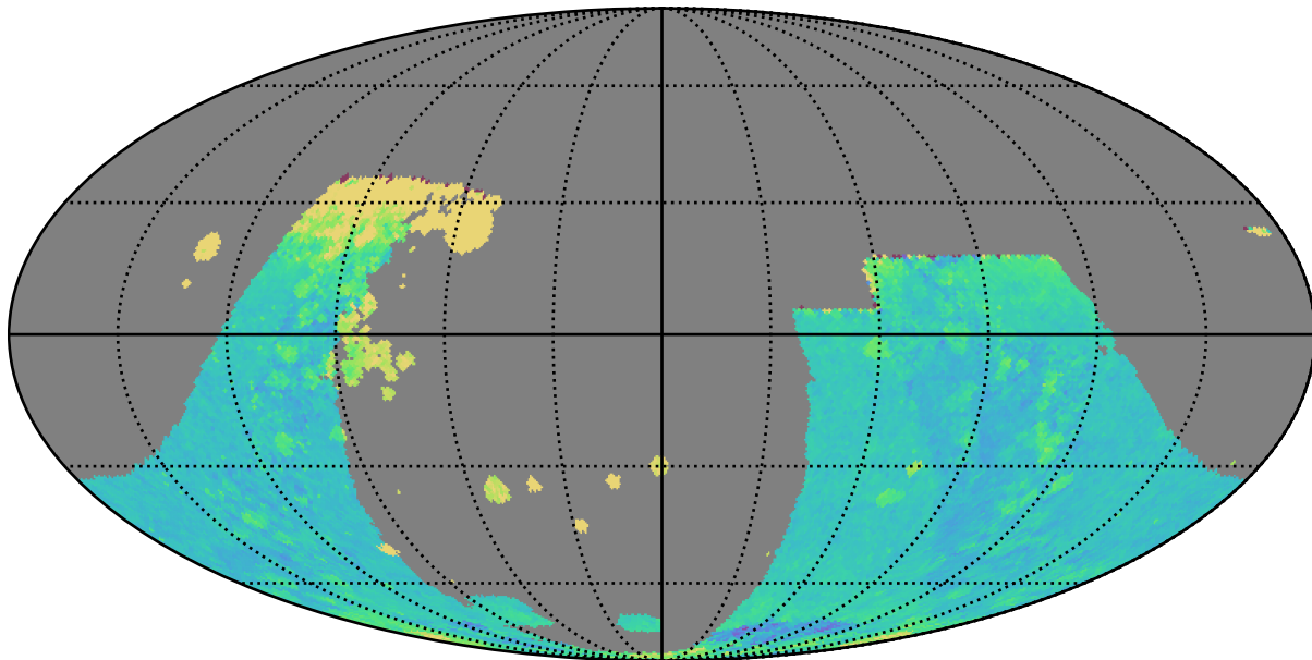
baseline_v3.3_10yrs : GalplaneTimePerFilter_combined_map_z
