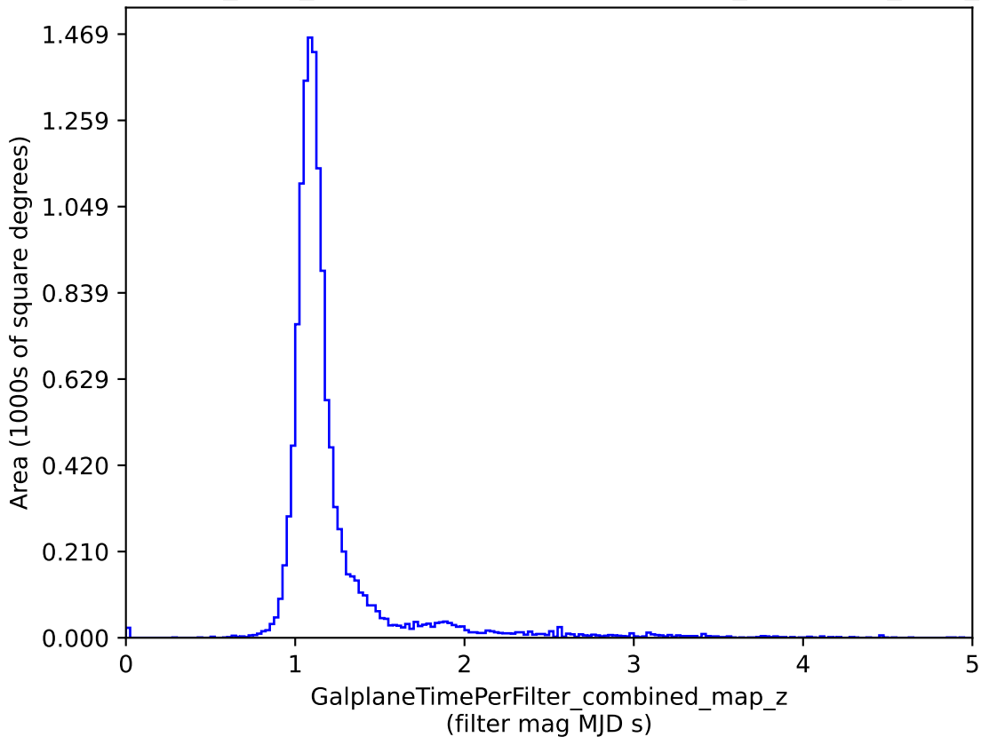
baseline_v3.3_10yrs : GalplaneTimePerFilter_combined_map_z
