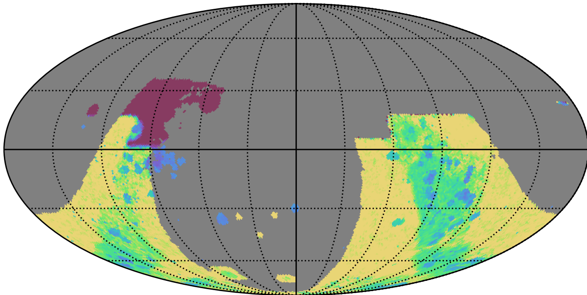
baseline_v3.3_10yrs : GalplaneTimePerFilter_combined_map_y
