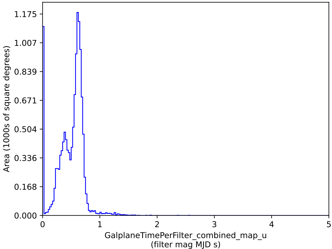
baseline_v3.3_10yrs : GalplaneTimePerFilter_combined_map_u
