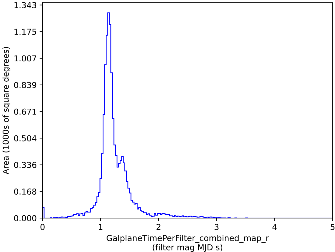
baseline_v3.3_10yrs : GalplaneTimePerFilter_combined_map_r
