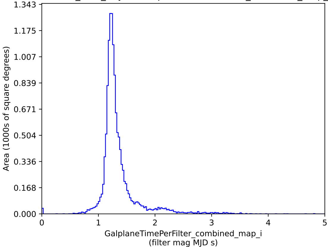
baseline_v3.3_10yrs : GalplaneTimePerFilter_combined_map_i
