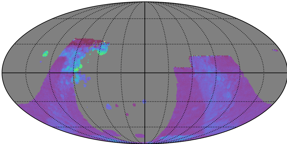
baseline_v3.3_10yrs : GalplaneTimePerFilter_combined_map_g
