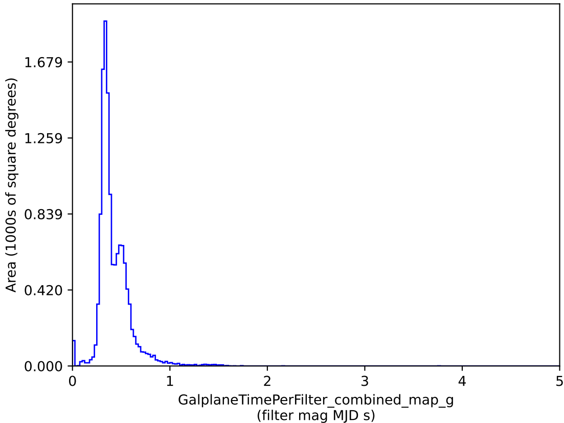
baseline_v3.3_10yrs : GalplaneTimePerFilter_combined_map_g
