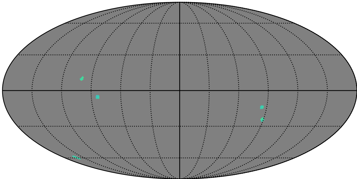
baseline_v3.3_10yrs : GalplaneTimePerFilter_bonito_sfr_map_z
