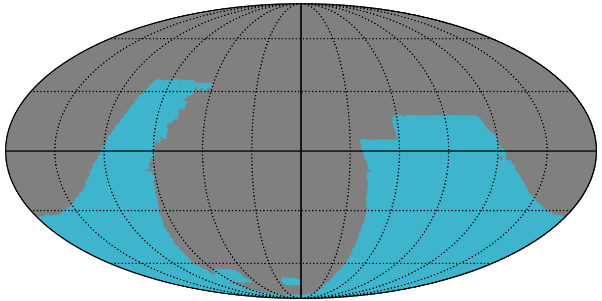
baseline_v3.3_10yrs : GalplaneFootprintMetric_galactic_plane_map_Tau_2_0
