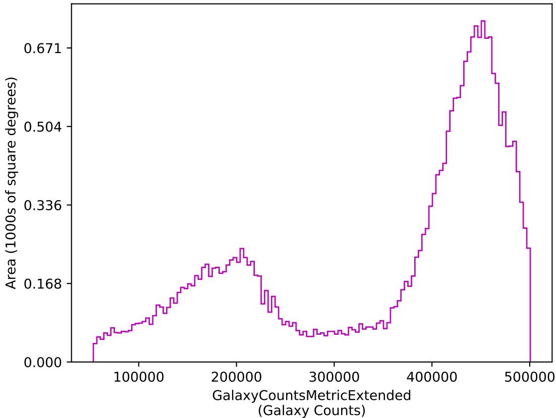
baseline_v3.3_10yrs z: GalaxyCountsMetricExtended
