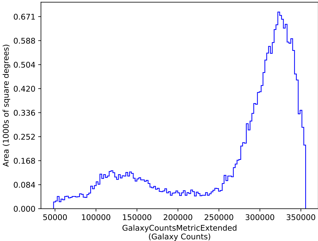
baseline_v3.3_10yrs y: GalaxyCountsMetricExtended
