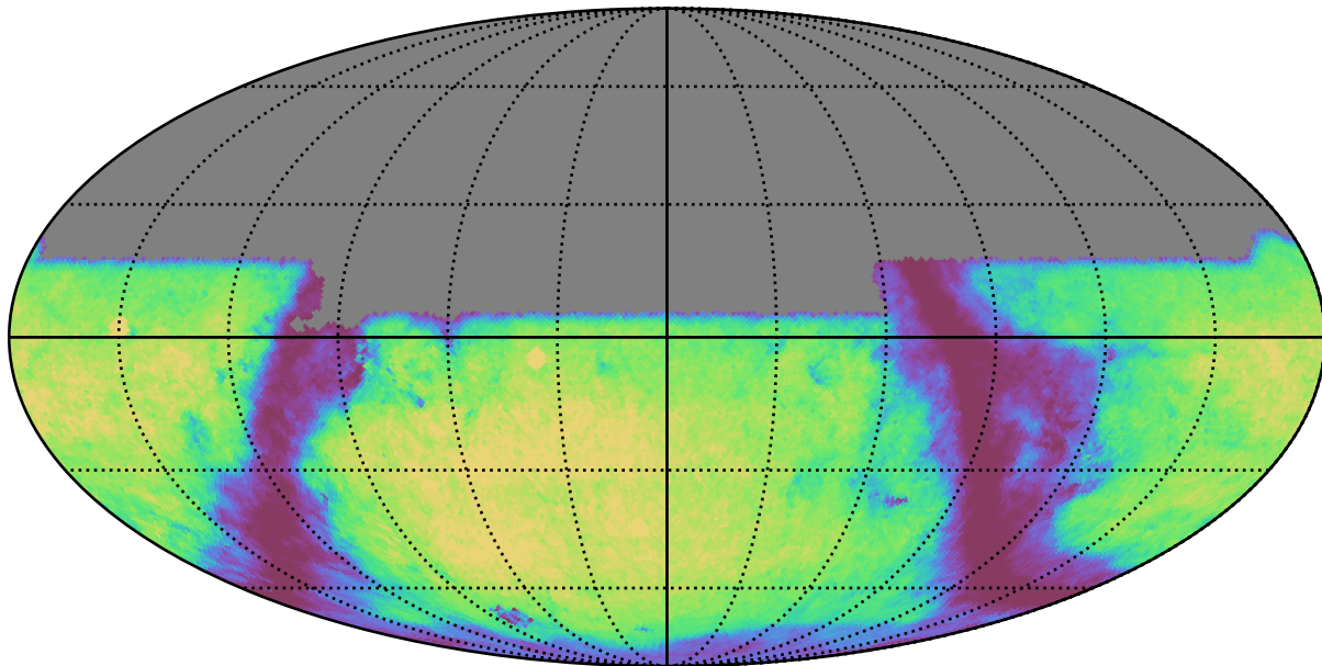
baseline_v3.3_10yrs u: GalaxyCountsMetricExtended
