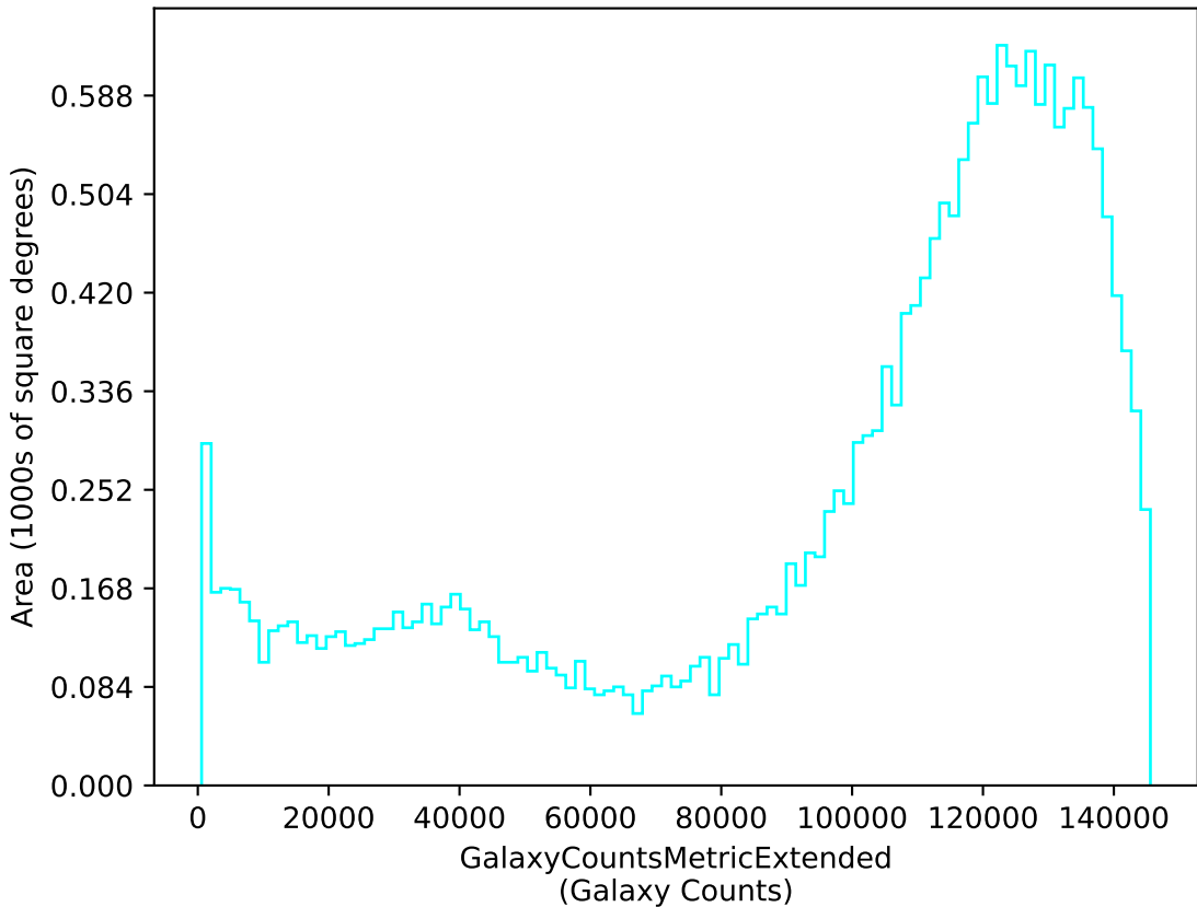
baseline_v3.3_10yrs u: GalaxyCountsMetricExtended
