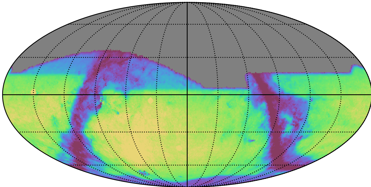
baseline_v3.3_10yrs r: GalaxyCountsMetricExtended
