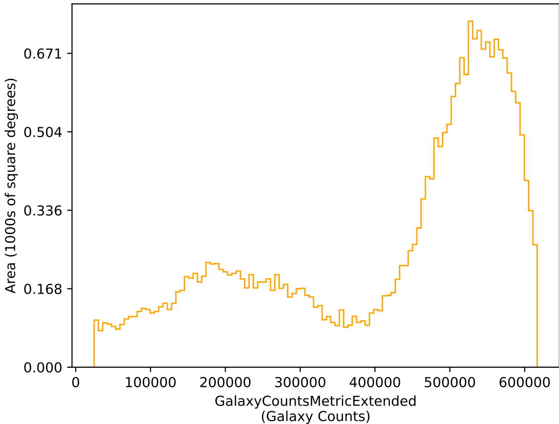
baseline_v3.3_10yrs r: GalaxyCountsMetricExtended
