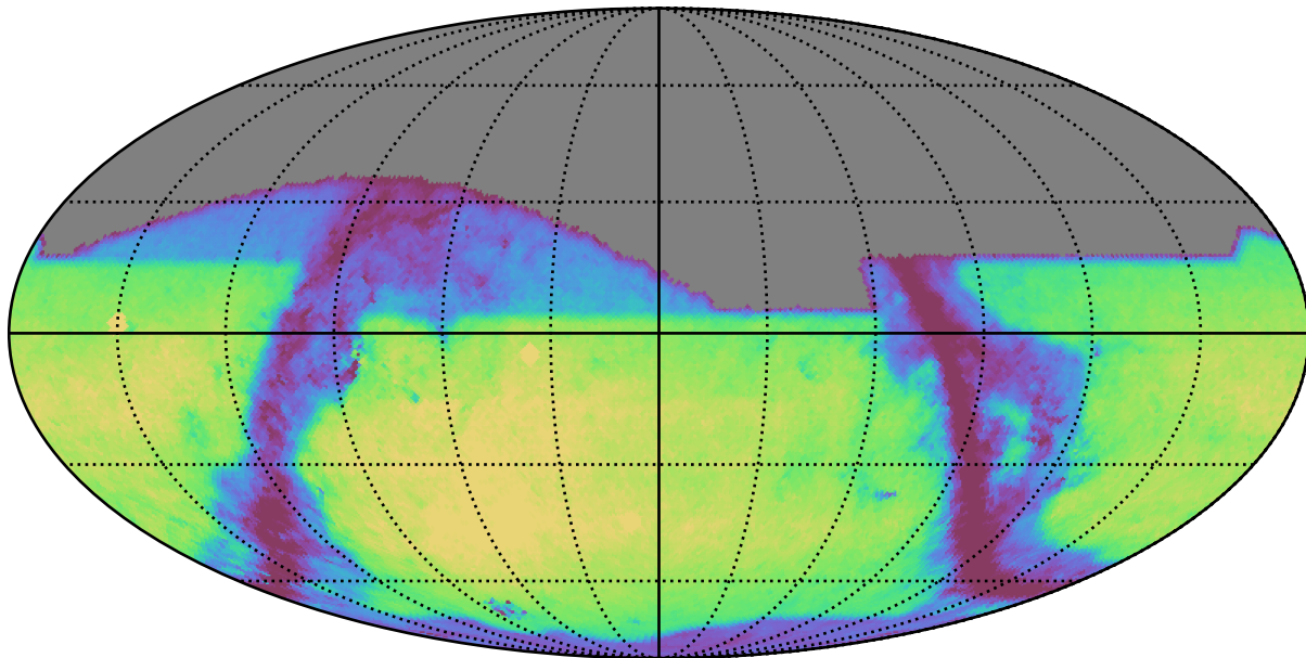
baseline_v3.3_10yrs i: GalaxyCountsMetricExtended
