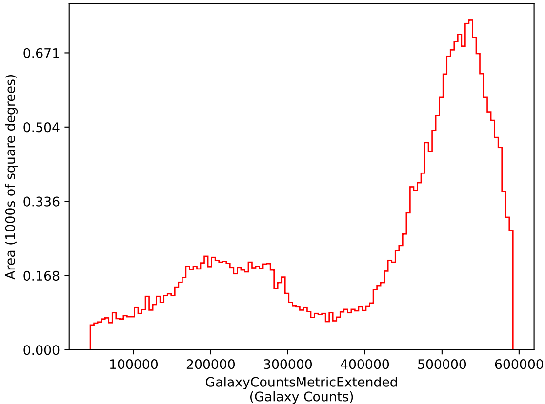
baseline_v3.3_10yrs i: GalaxyCountsMetricExtended
