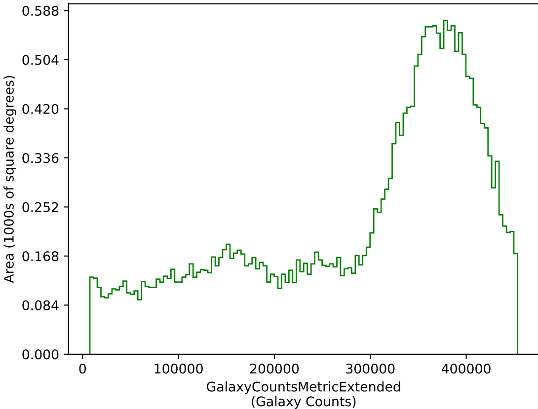
baseline_v3.3_10yrs g: GalaxyCountsMetricExtended
