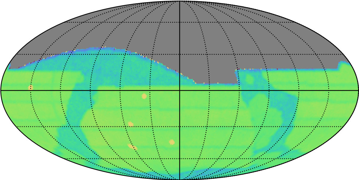
baseline_v3.3_10yrs : GalPlaneVisitIntervalsTimescales_xray_binaries_map_Tau_2_0
