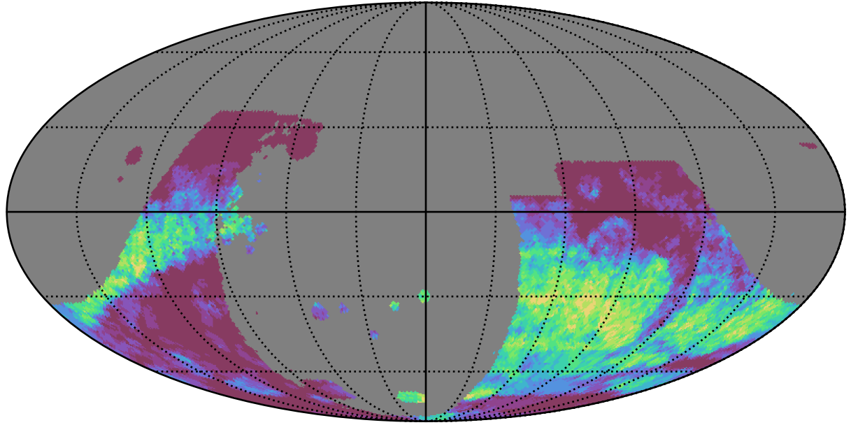
baseline_v3.3_10yrs : GalPlaneSeasonGapsTimescales_combined_map_Tau_25_0
