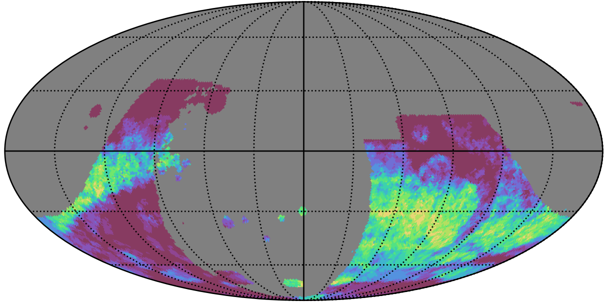
baseline_v3.3_10yrs : GalPlaneSeasonGapsTimescales_combined_map_Tau_10_0
