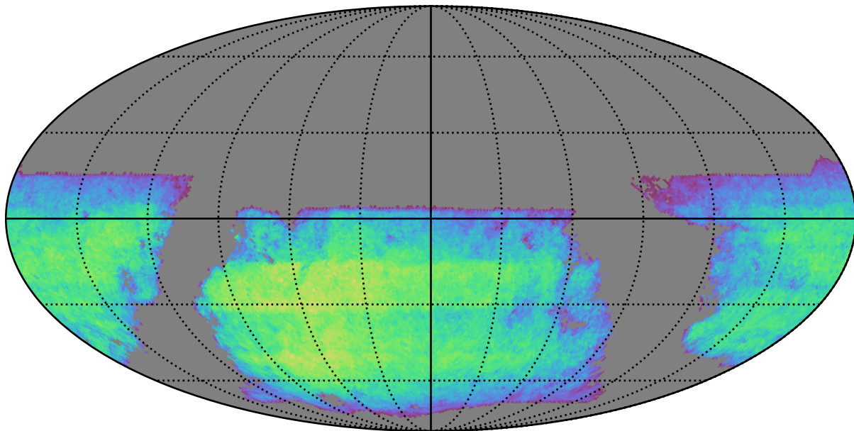
baseline_v3.3_10yrs i band non-DD year 9: ExgalM5WithCuts
