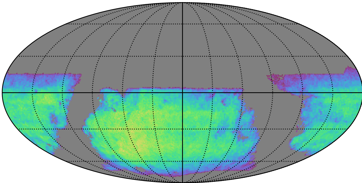
baseline_v3.3_10yrs i band non-DD year 8: ExgalM5WithCuts
