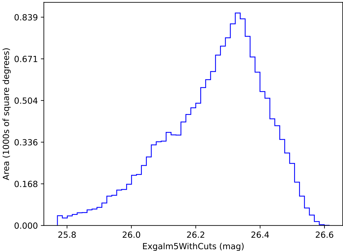
baseline_v3.3_10yrs i band non-DD year 8: ExgalM5WithCuts
