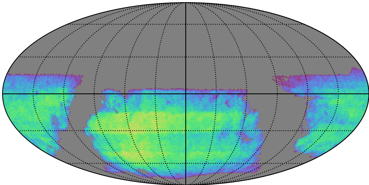
baseline_v3.3_10yrs i band non-DD year 7: ExgalM5WithCuts
