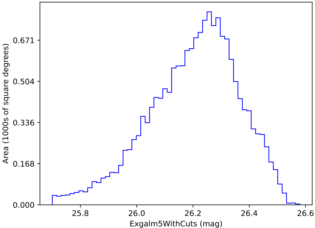
baseline_v3.3_10yrs i band non-DD year 7: ExgalM5WithCuts
