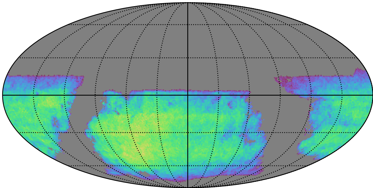
baseline_v3.3_10yrs i band non-DD year 6: ExgalM5WithCuts
